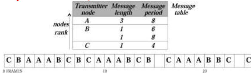
Fig. 1. Example of implicit contention using EDF.
