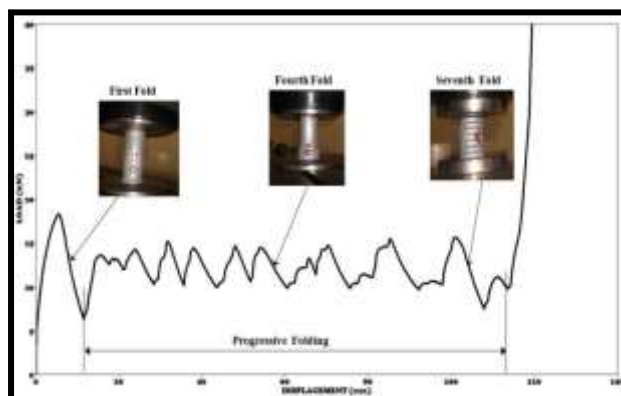
Figure 9 Typical Load-displacement curve when the aluminium tube compressed under quasi-static loading condition.
