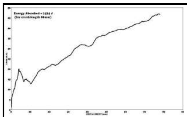
Figure 8 Load-displacement curve for the aluminium tube specimen (6mm)
