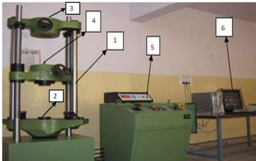
Figure 3: Electronic universal testing machine
