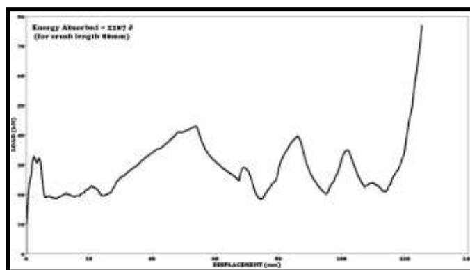
Figure6 Load-displacement curve for the aluminium tube specimen (4mm)
