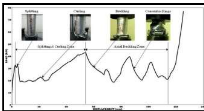
Figure 5 Typical load-displacement curve when aluminium tube compressed under quasi static loading condition (4mm)
