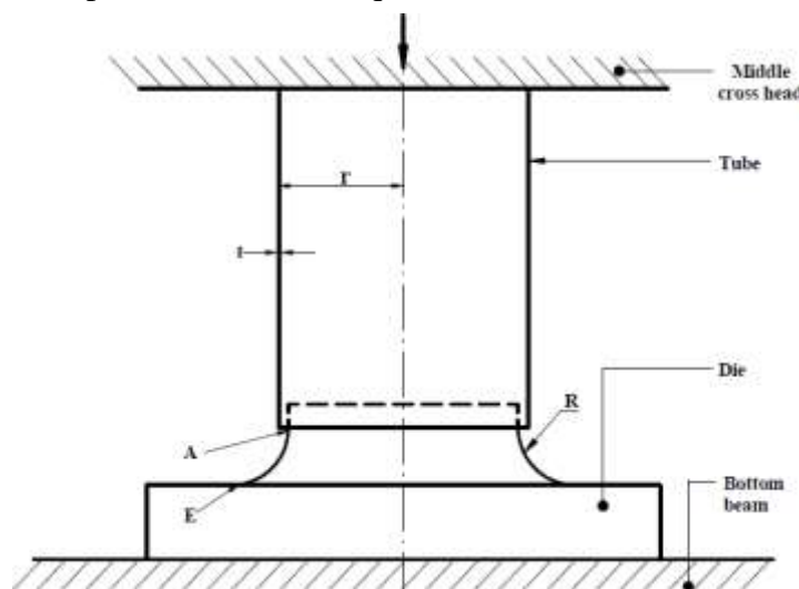
Figure4 Schematic of the test set up
