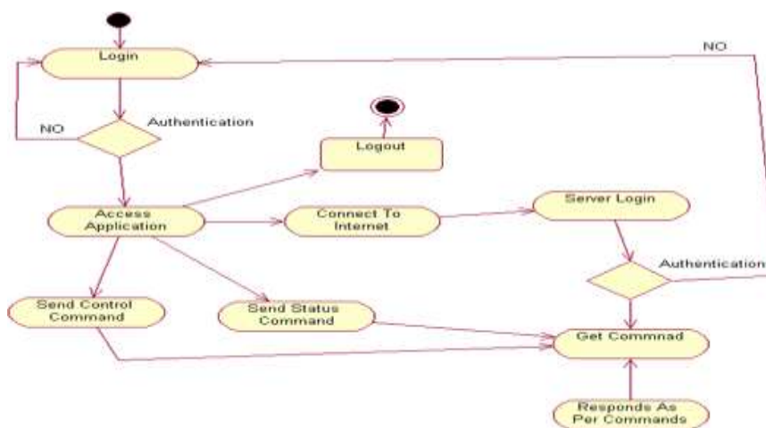
Fig.5.1.1. Communication Flow with the Server
