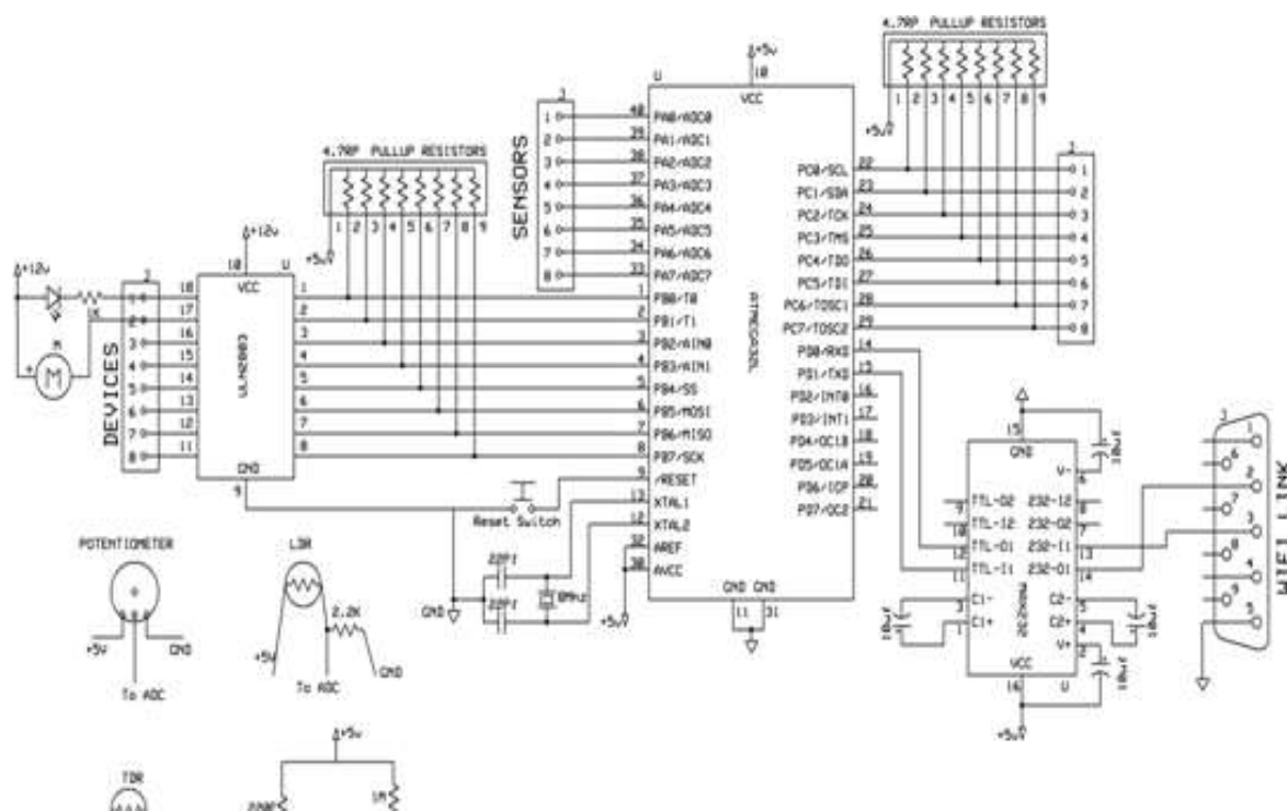
Fig.2.1. Circuit Diagram of the System
