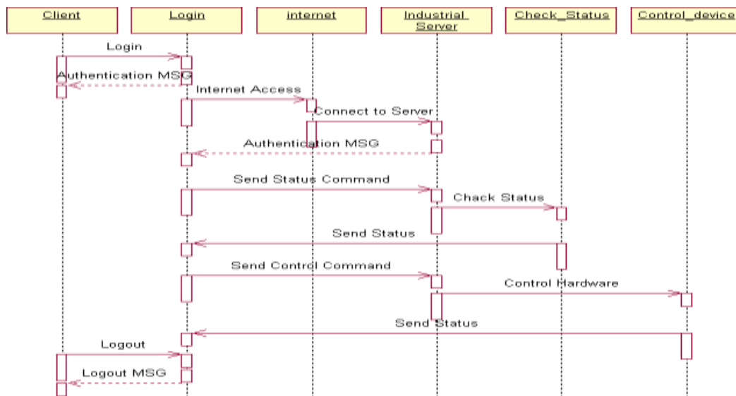
Fig.5.2.1. Server Authentication Flow
