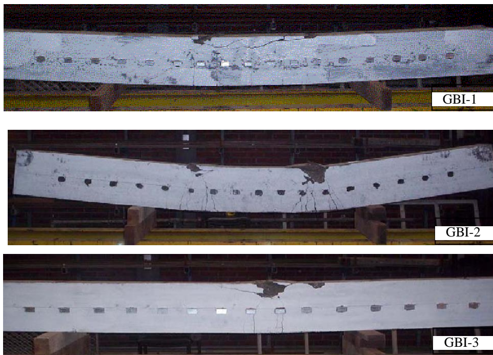
Figure 2 – Beams after test
