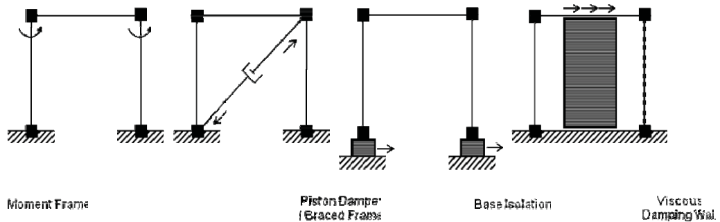
Figure 3: Options for Structural Systems
