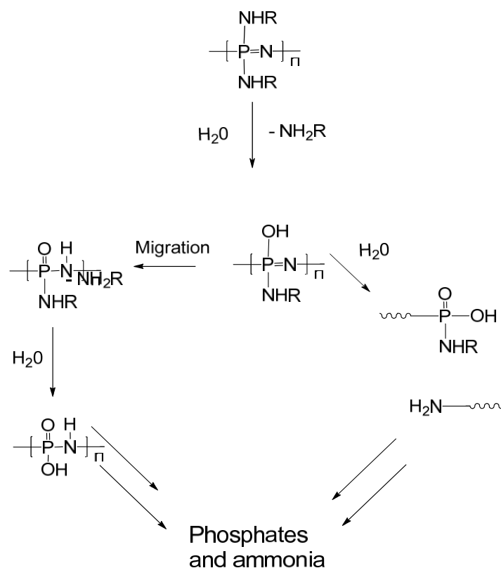
Figure 5. Non-catalyzed mechanism for the degradation of poly[(organo)phosphazenes].
