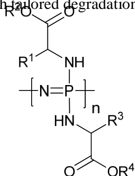
Figure 7. Generic structure for amino acid ester substituted poly[(organo)phosphazenes]. R 1 -R 4 can be varied to give a range of poly[(organo)phosphazenes] with tailored degradation rates.
