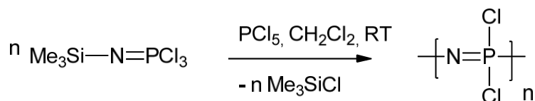
Figure 4. The living cationic polymerization route to polydichlorophosphazene.
