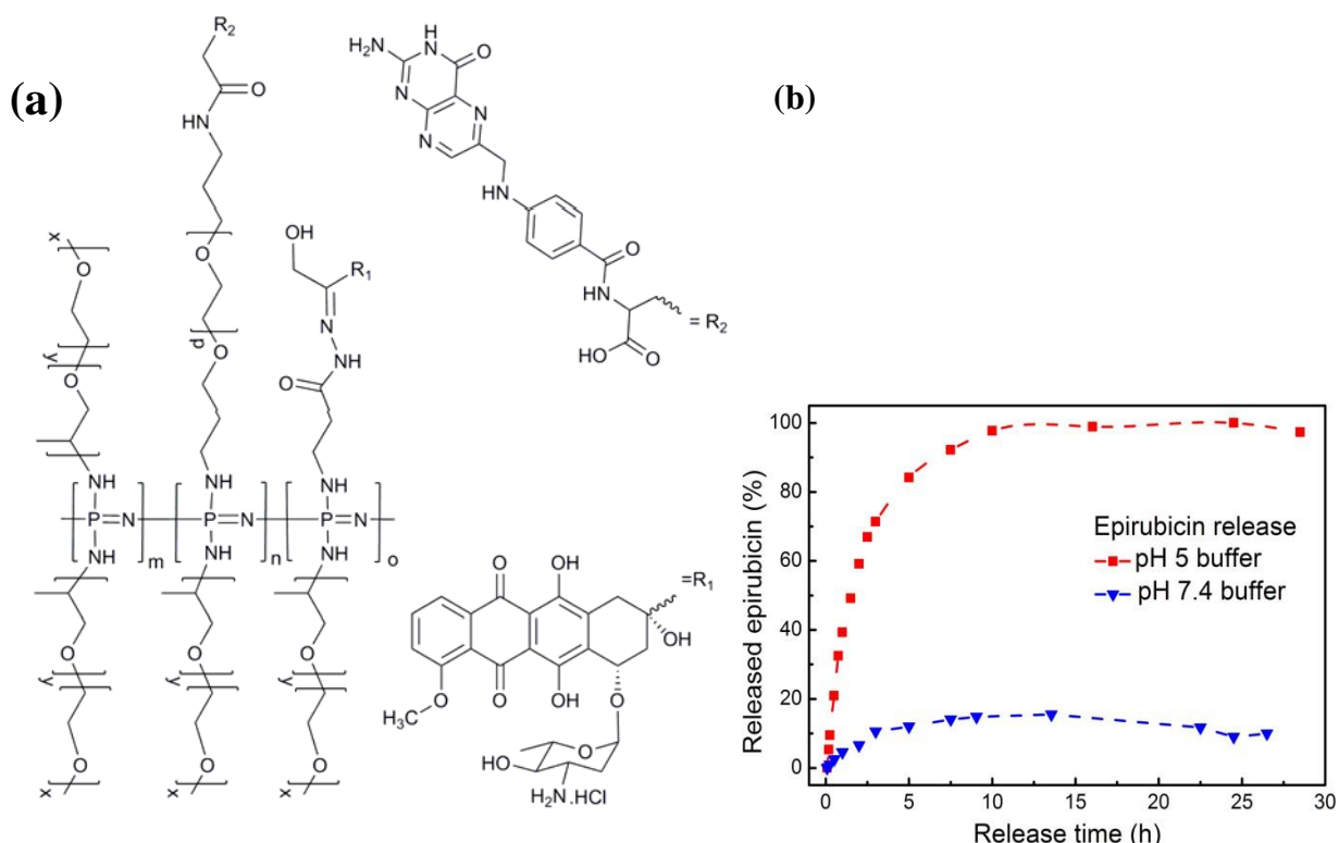
Figure 11. (a) Water soluble polyphosphazene loaded with a folic acid targeting ligands and epirubicin via a pH labile hydrazone bond. (b) Release of epirubicin from the hydrazone-linked polyphosphazene pH 5 (■) and pH 7.4 (▼). Originally published in [29] and reproduced by permission of The Royal Society of Chemistry.
