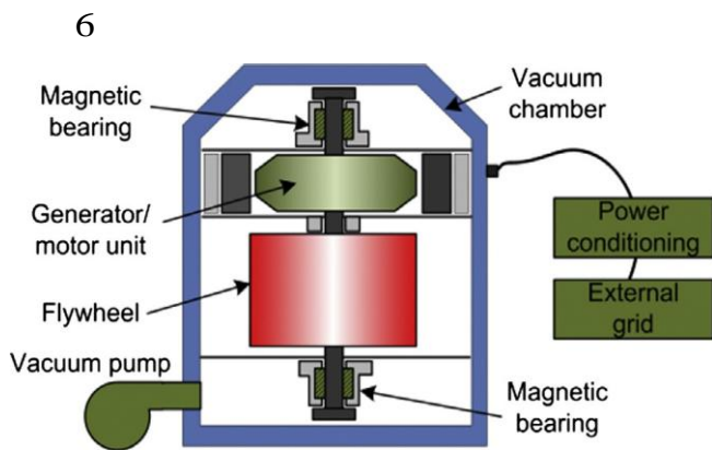
Fig. 6. System description of a flywheel energy storage facility.
