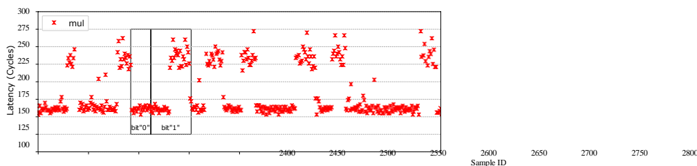
Fig. 15. Access latencies measured in the probe operation in Prime+Probe. A sequence of "01010111011001" can be deduced as part of the exponent.
