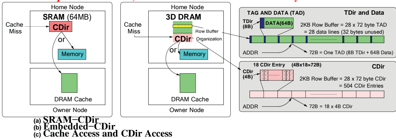
Fig. 7. Coherence Directory Organization. (a) SRAM-based Coherence Directory, (b) Embedded Coherence Directory and (c) Cache Access and CDir Access. One read access to Embedded-CDir in 3D DRAM gets 18 CDir entries (72 bytes). Note that our proposal is based on, but not limited to, Alloy Cache [15].
