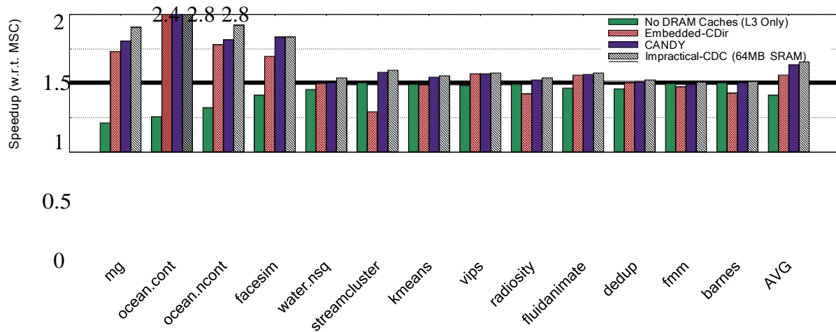
Fig. 15. Performance of No DRAM Caches (L3 Only), Embedded-CDir, our proposed CANDY, and impractical CDC with 64MB SRAM overhead and zero L4 cache read latency for RFD operation (Impractical-CDC). Note that the performance is normalized to the baseline Memory-Side Cache. We report the geometric mean as an AVG in the right most bar.
