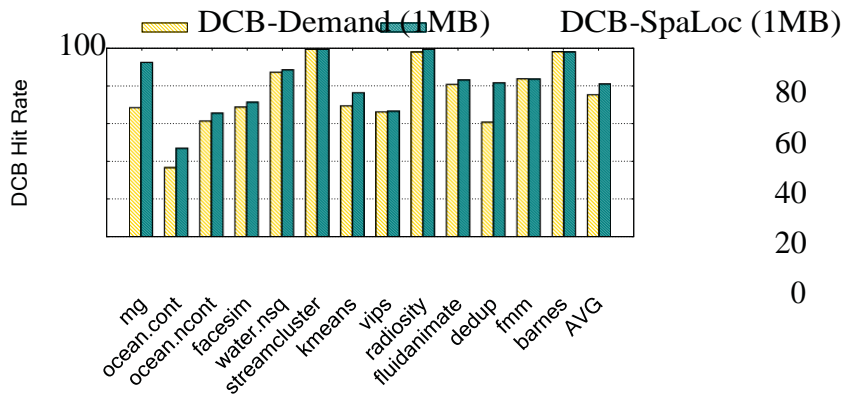
Fig. 11. DCB Hit Rate: DCB-Demand and DCB-SpaLoc. Both are allowed for 1MB SRAM in size.
