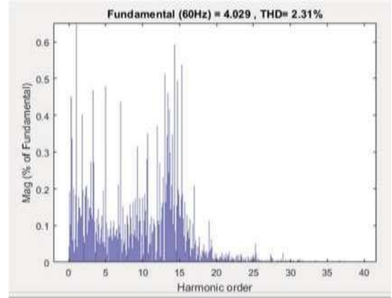
Fig. 12. Harmonic spectrum and THD of grid-injected current
