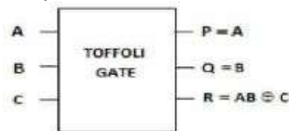
Figure 3.2 Toffoli gate
