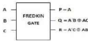
Figure 3.3 Fredkin gate
