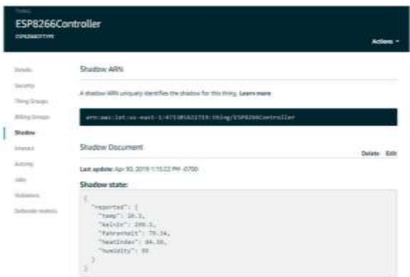
Figure 8: AWS IoT Core Shadow
