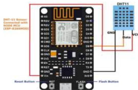
Figure 4: Block diagram and connections
