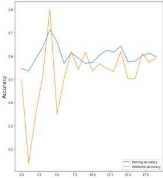
Fig.7 The accuracy of PCA net
