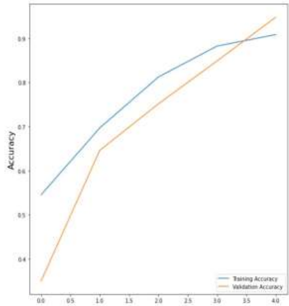
Fig.5 The accuracy of mobile net Fig.5 Shows that the accuracy between the training accuracy and validation accuracy.
