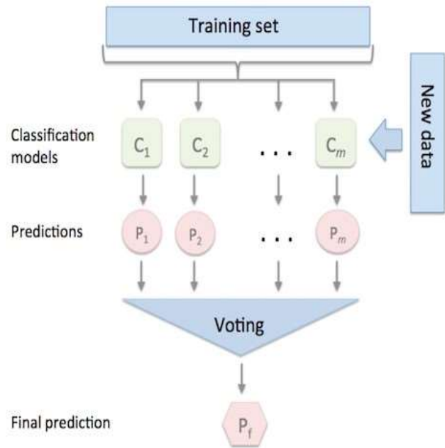
Fig.2 Voting Classifier
