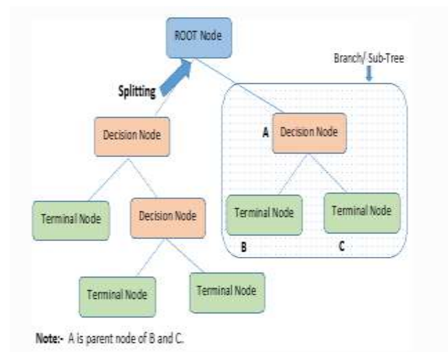
Fig.3 Decision tree
