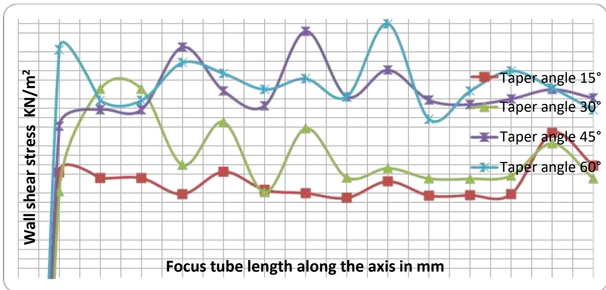
Figure 5 (b) Wall shear stress along focus tube
