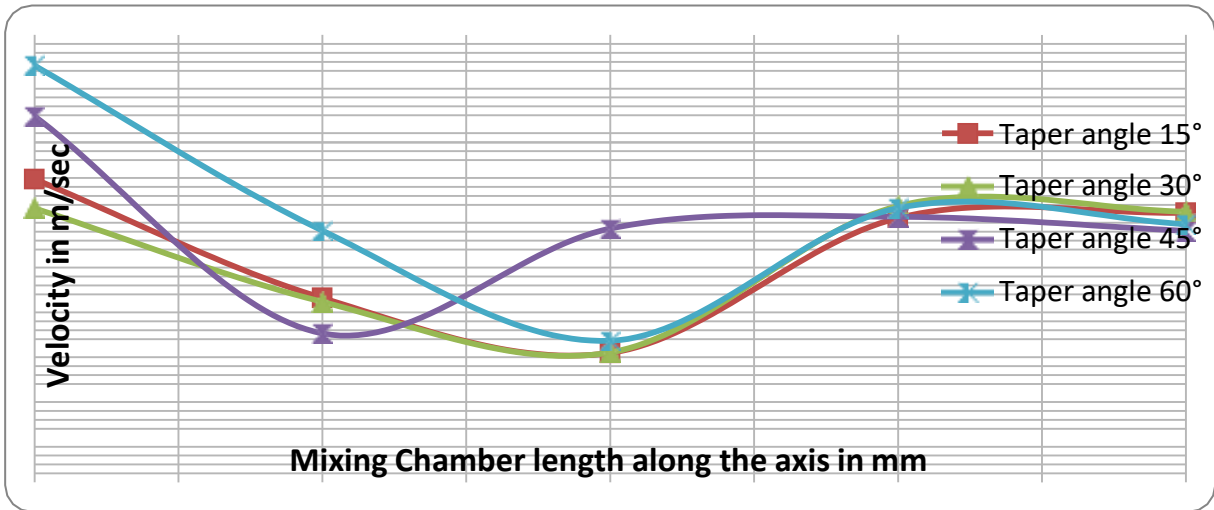
Figure 4 (a) Velocity variation along the Mixing Chamber
