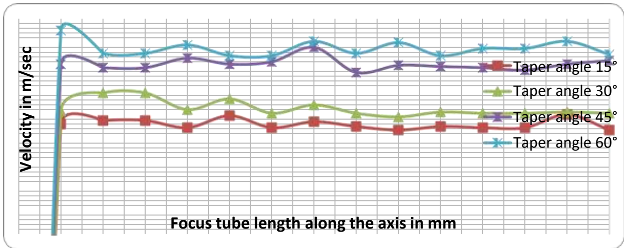
Figure 4 (b) Velocity variation along the Focus tube
