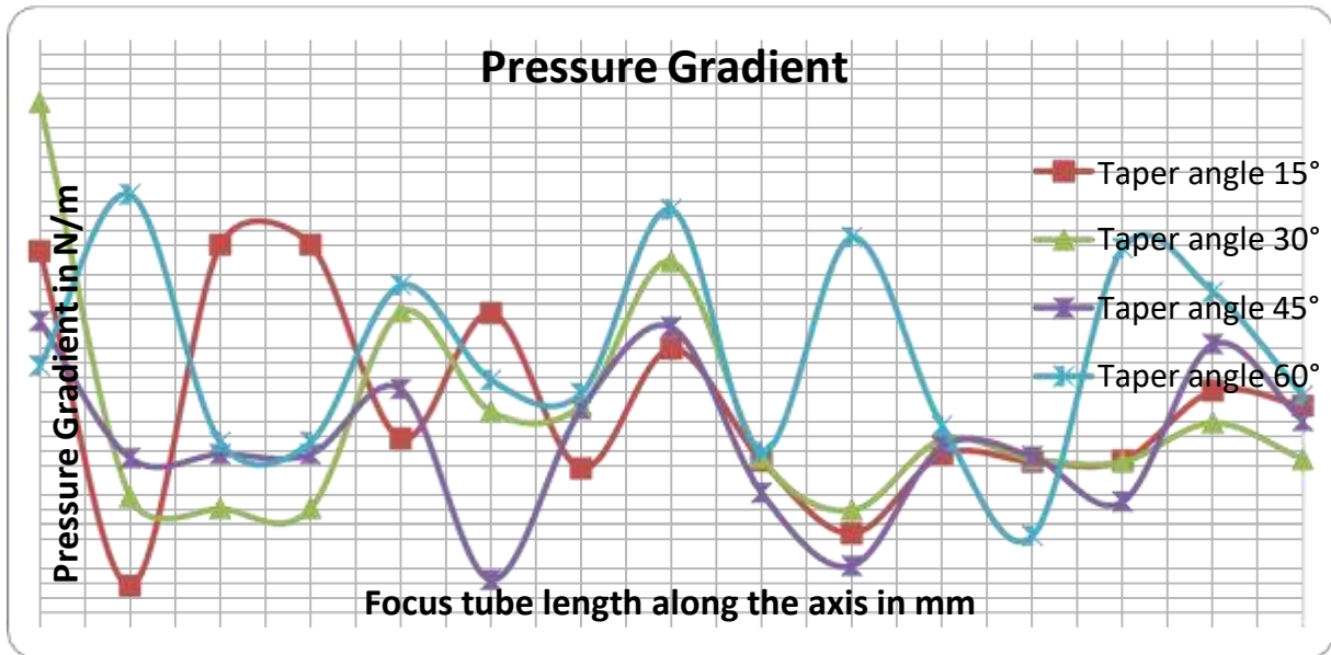
Figure 6 (b) Pressure gradient in the focus tube
