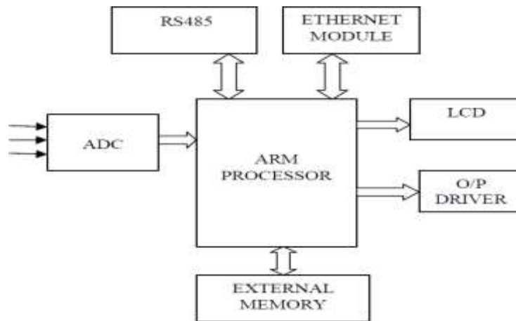
Fig -2: Embedded web server for real time application
